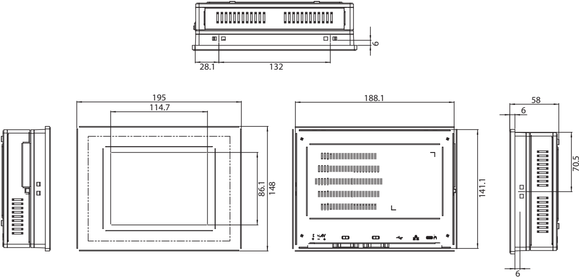
Panel Cut-out Dimensions: 189.1 x 142.1 mm (7.56" x 5.68")
